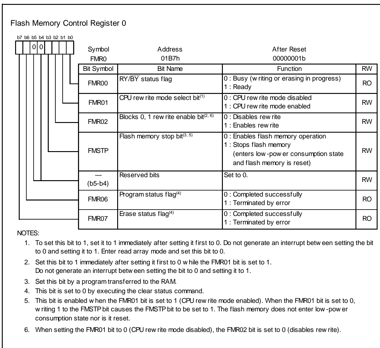
Figure 20.5 FMR0 Register
