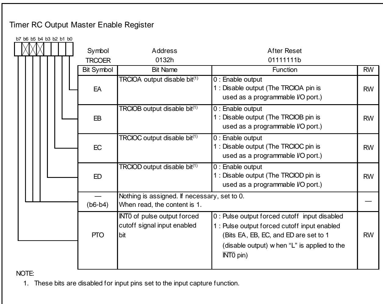
Figure 14.35 TRCOER Register
